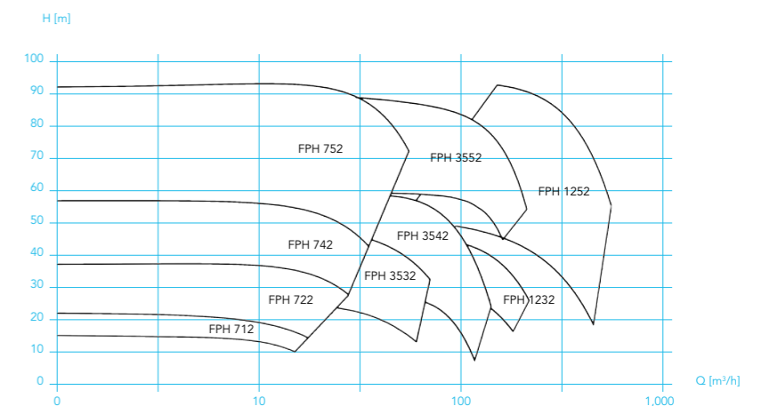
Characteristic curves of the Fristam series FPH; n = 2,900 min -1
